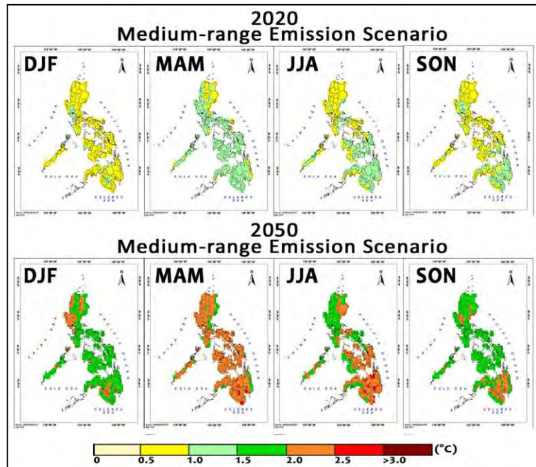
Fig.17: Maps showing the projected seasonal temperature increase (in °C) in the Philippines in 2020 and 2050.
